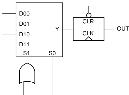
Figure 6 • Sequential Logic Module
