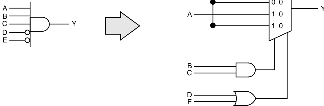
Figure 5 • Example of a Logic Function Implemented with the Combinatorial Logic Module
