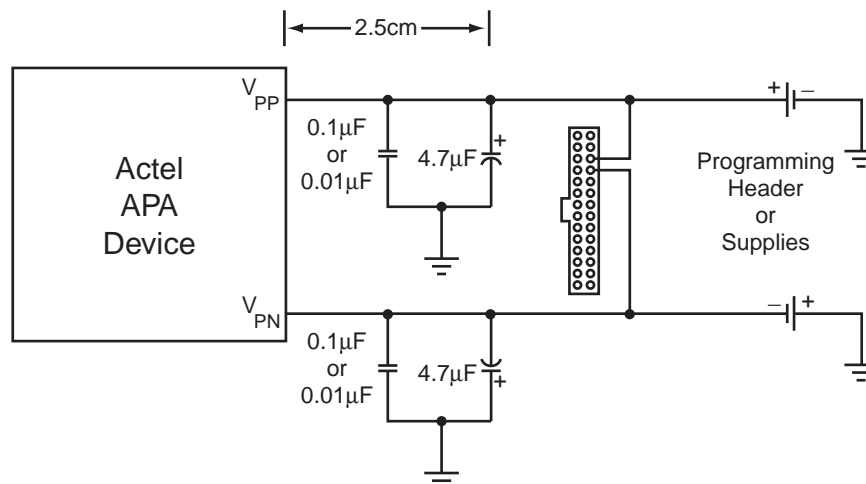
Figure 6 • V PP and V PN Capacitor Requirements
