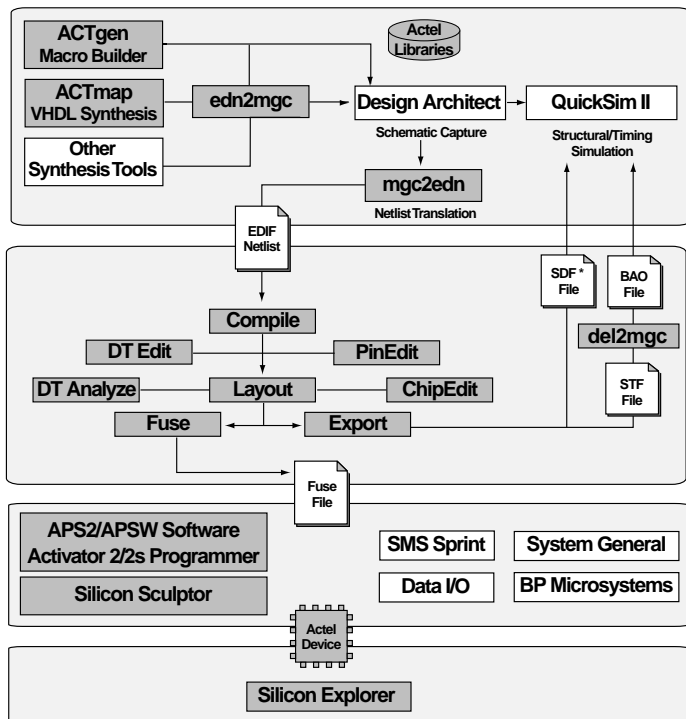
Figure 2-1. Schematic-Based Design Flow
