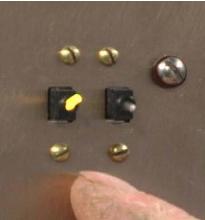
Soft ground switches (20-Ω)
