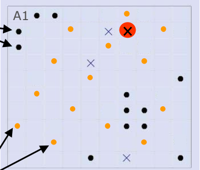
Stratix-II 2S60/F1020
